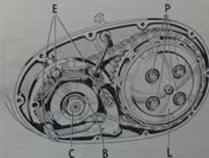
Fig. 12. Primary chain tensioner.
