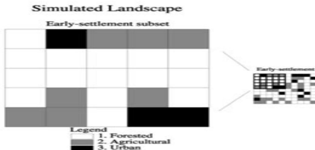
Figure 4.2 Subset of the early-settlement landscape used for calculating the Contagion index
