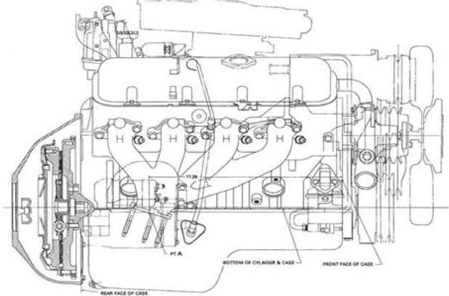
Figure 136 — Chevrolet big-block V8, right side.
