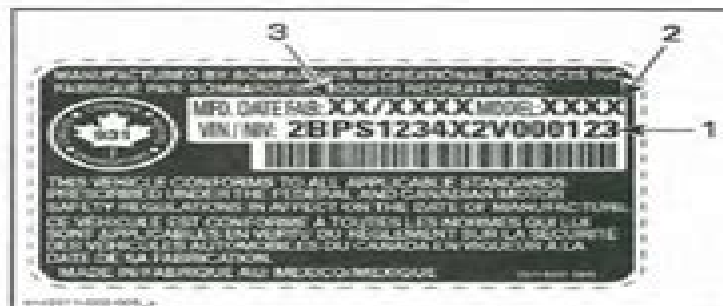
TYPICAL — VEHICLE IDENTIFICATION NUMBER LABEL 1. VIN (Vehicle Identification Number) 2. Model number 3. Manufacturing date
