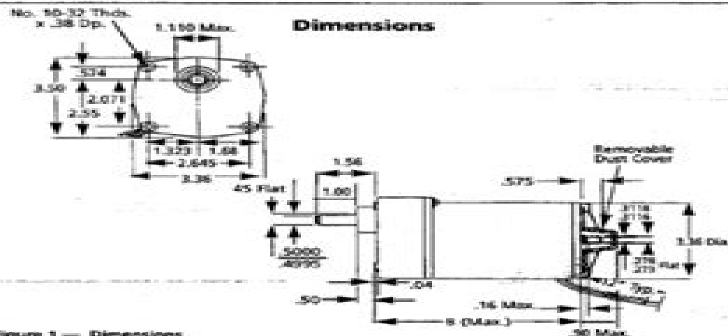
Figure 1 — Dimensions
