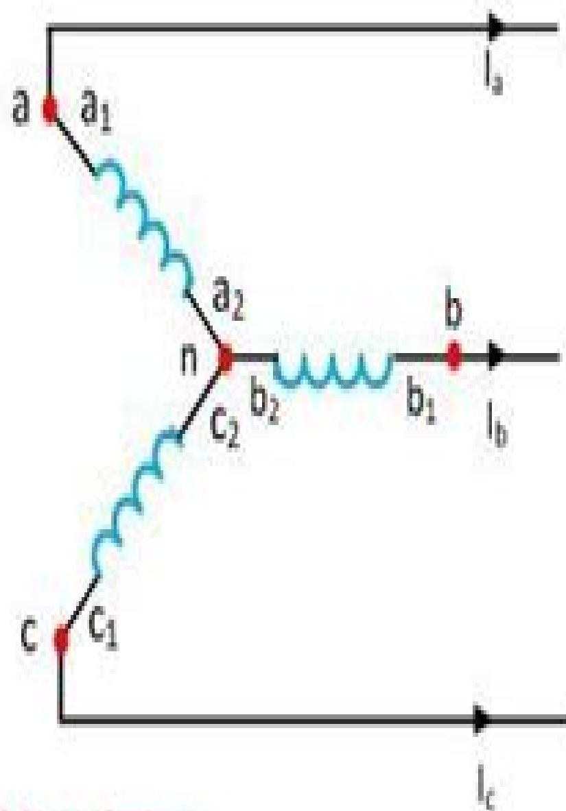
Delta Star Connection of Transformer
