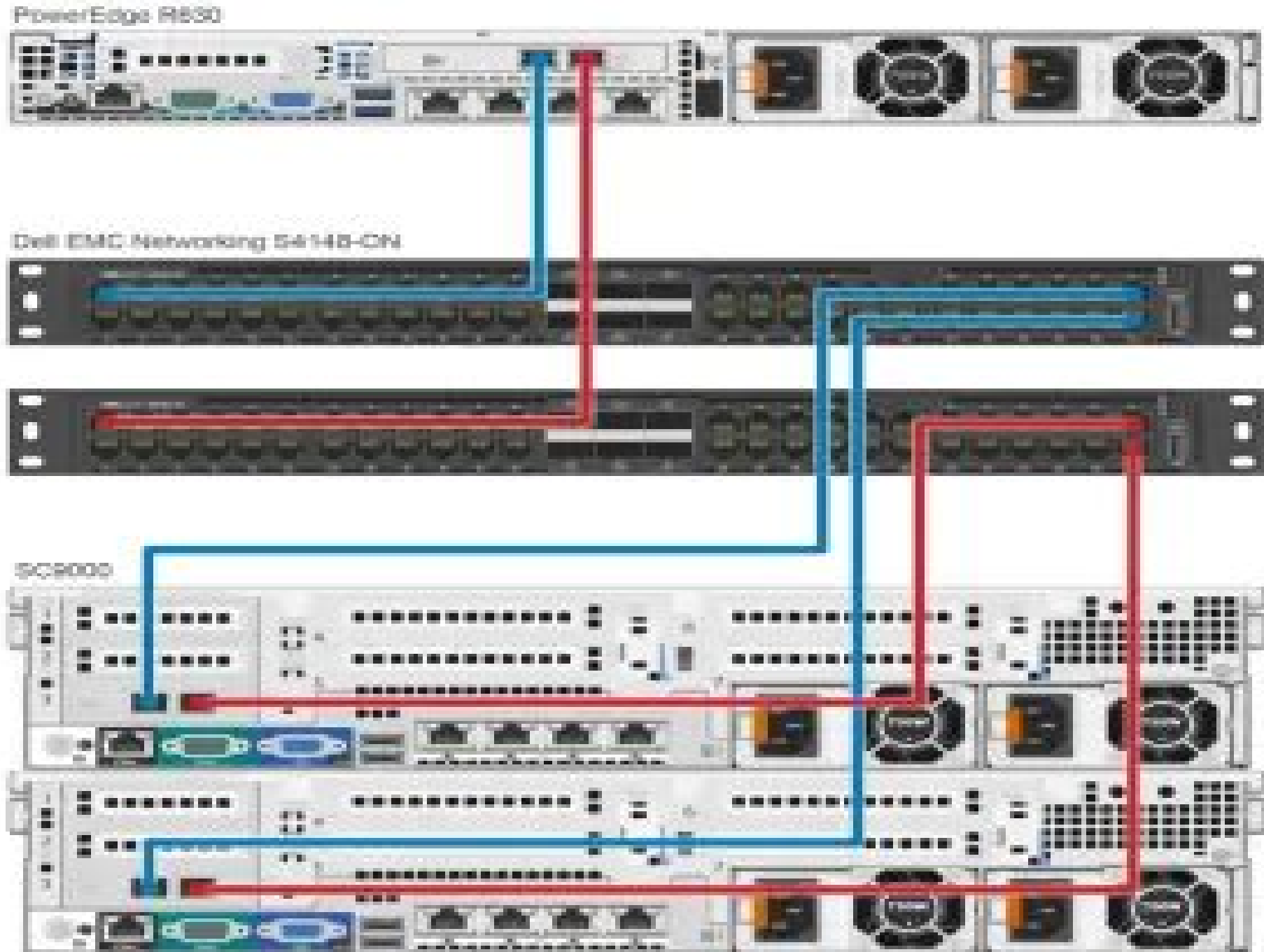
Figure 1 Cabling diagram
