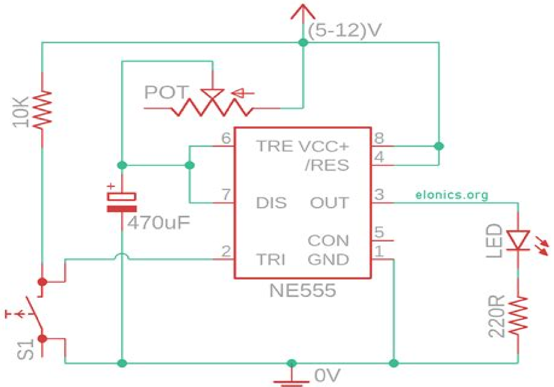
DELAY TIMER CIRCUIT SCHEMATIC
