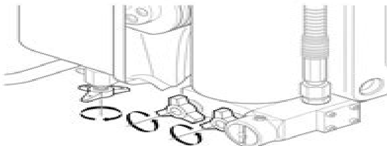
Fig. 8 Opening the condensate drain taps
