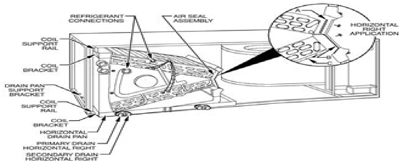
Fig. 6 - A-Coil in Horizontal-Right Application (FE4A only)
