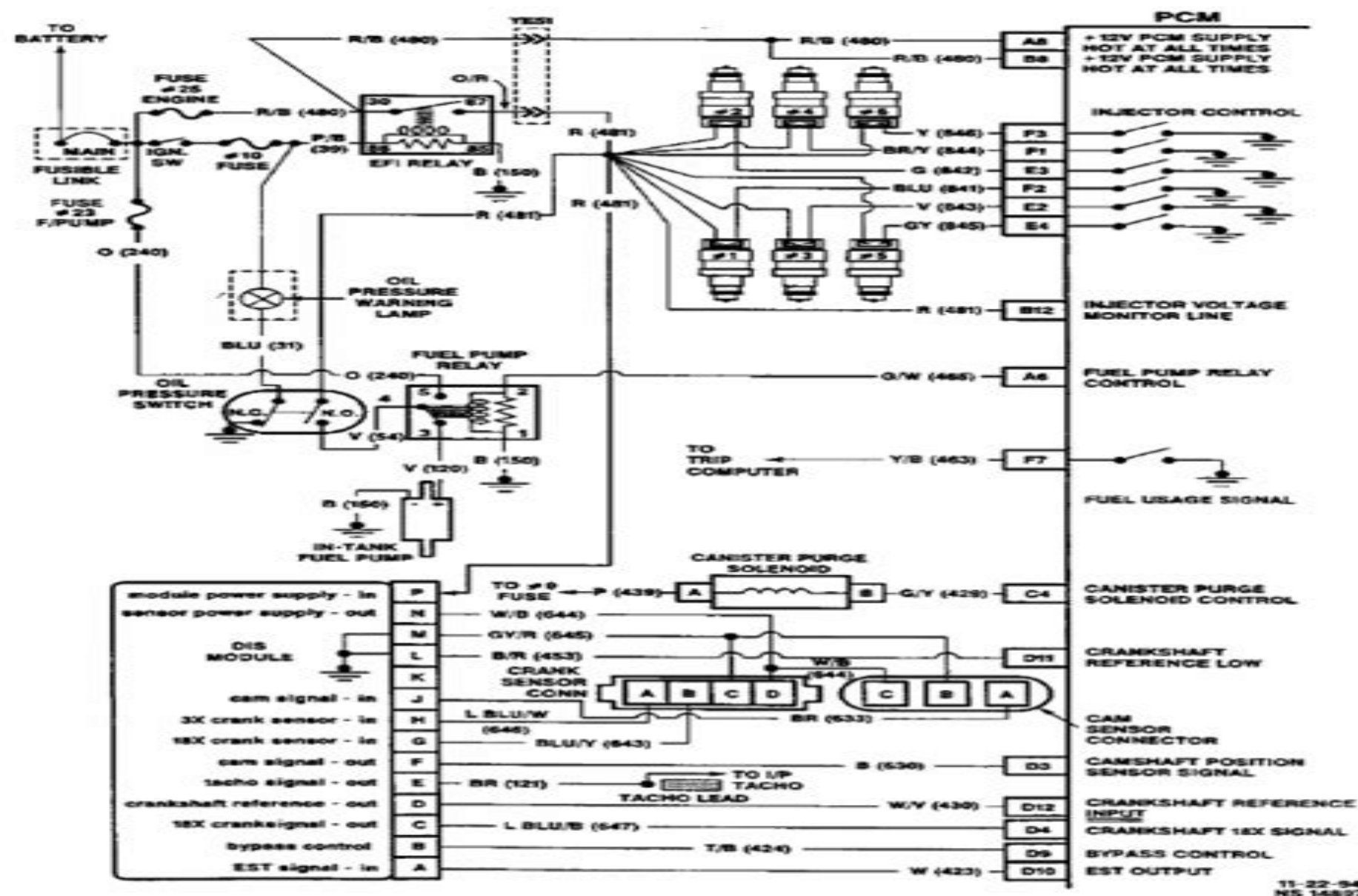
Figure 6C1-2A-5 V6 PCM Wiring Diagram (1 of 5)
