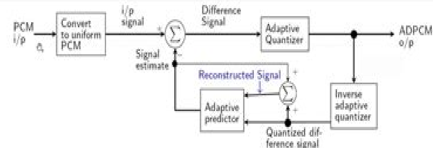
(a) Encoder
