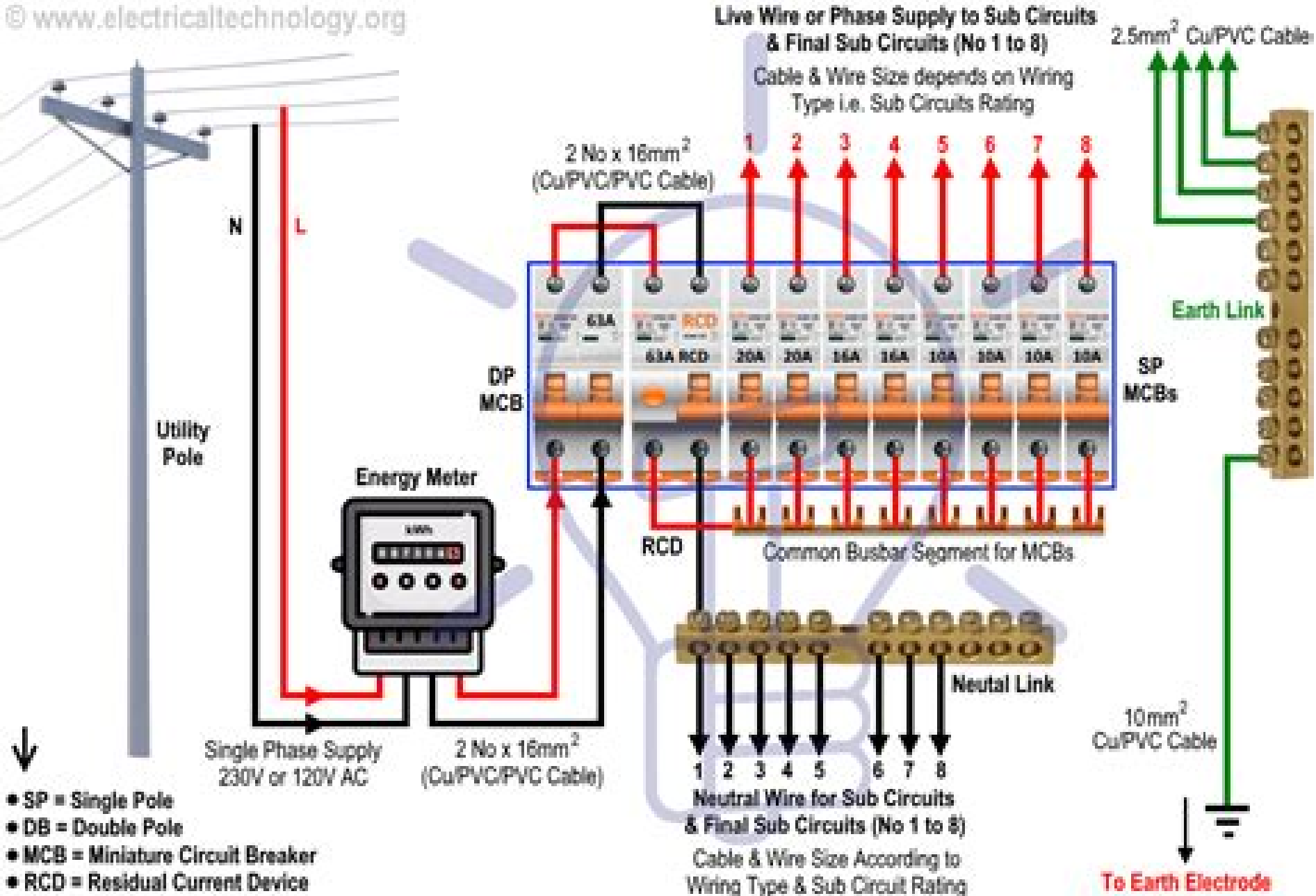
Wiring of the Distribution Board with RCD (Single Phase Supply) (From Utility Pole & Energy Meter to the Consumer Unit)
