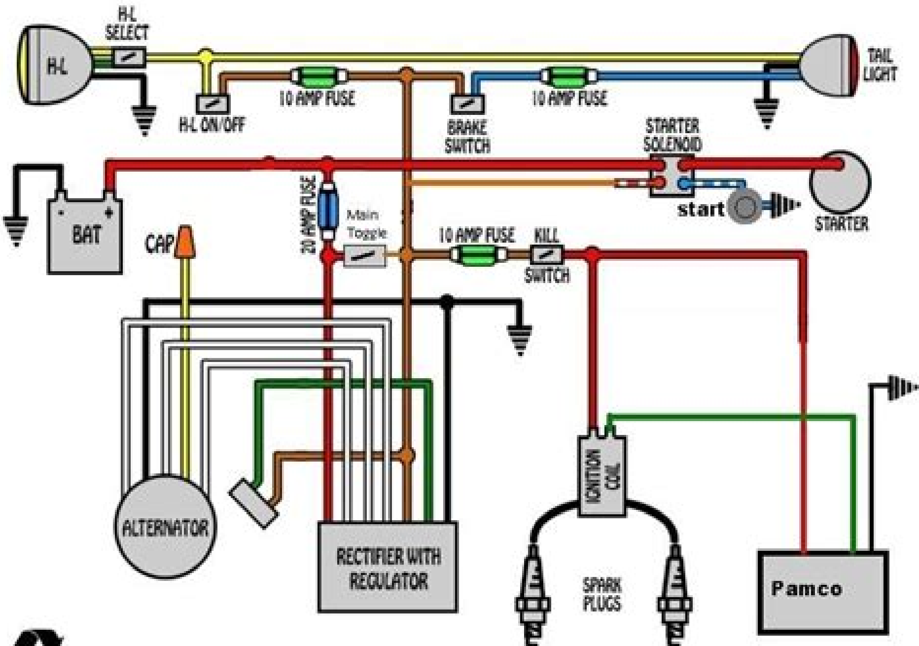
1980XS650 SIMPLIFIED AND COMPLETE WIRING DIAGRAM
