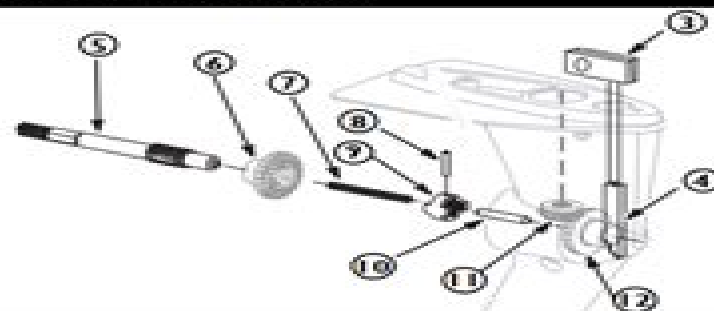
Figure 5 — Forward Gear
