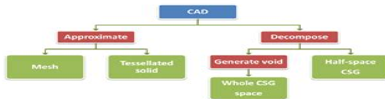
Fig 1.1 McCAd workflow
