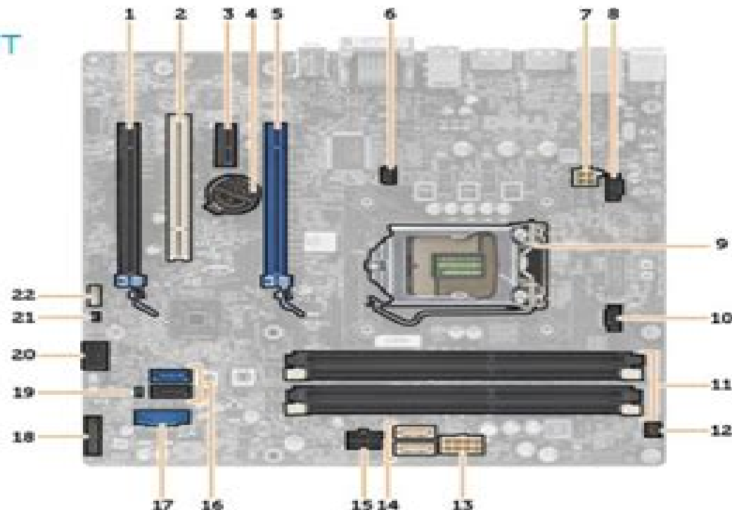
Figure 1. Components Of The System Board
