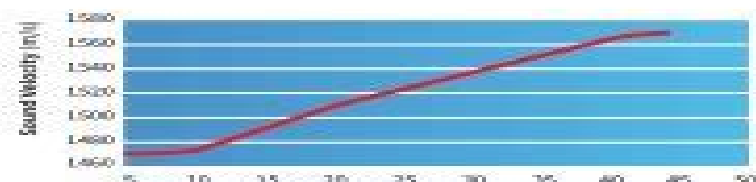
Sulphuric Acid 6..40% wt (25 Deg C)
