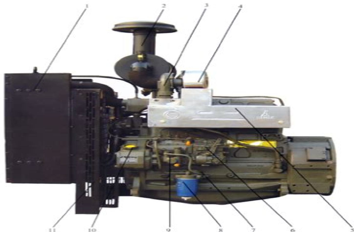
4-cylinder diesel engine
