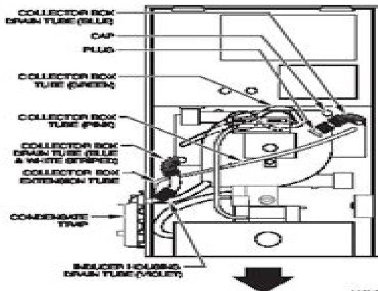
Fig. 9 - Downflow Tube Configuration (Left-Hand Trap Installation)
