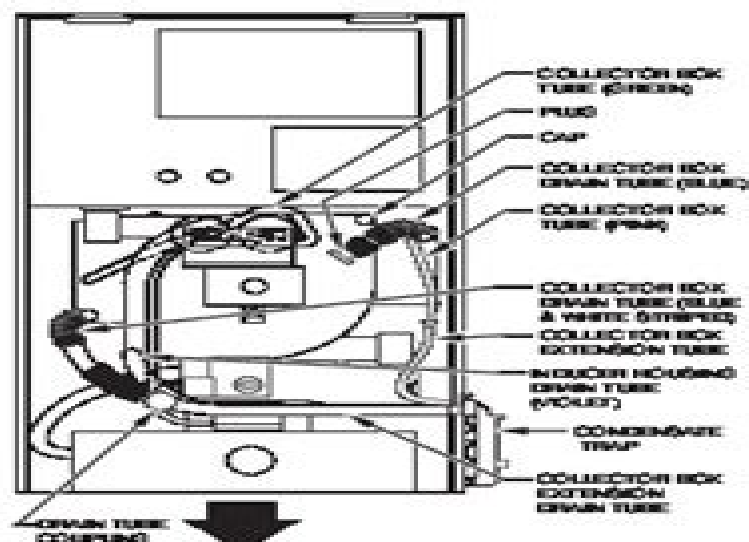
Fig. 10 - Downflow Tube Configuration (Right-Hand Trap Installation)
