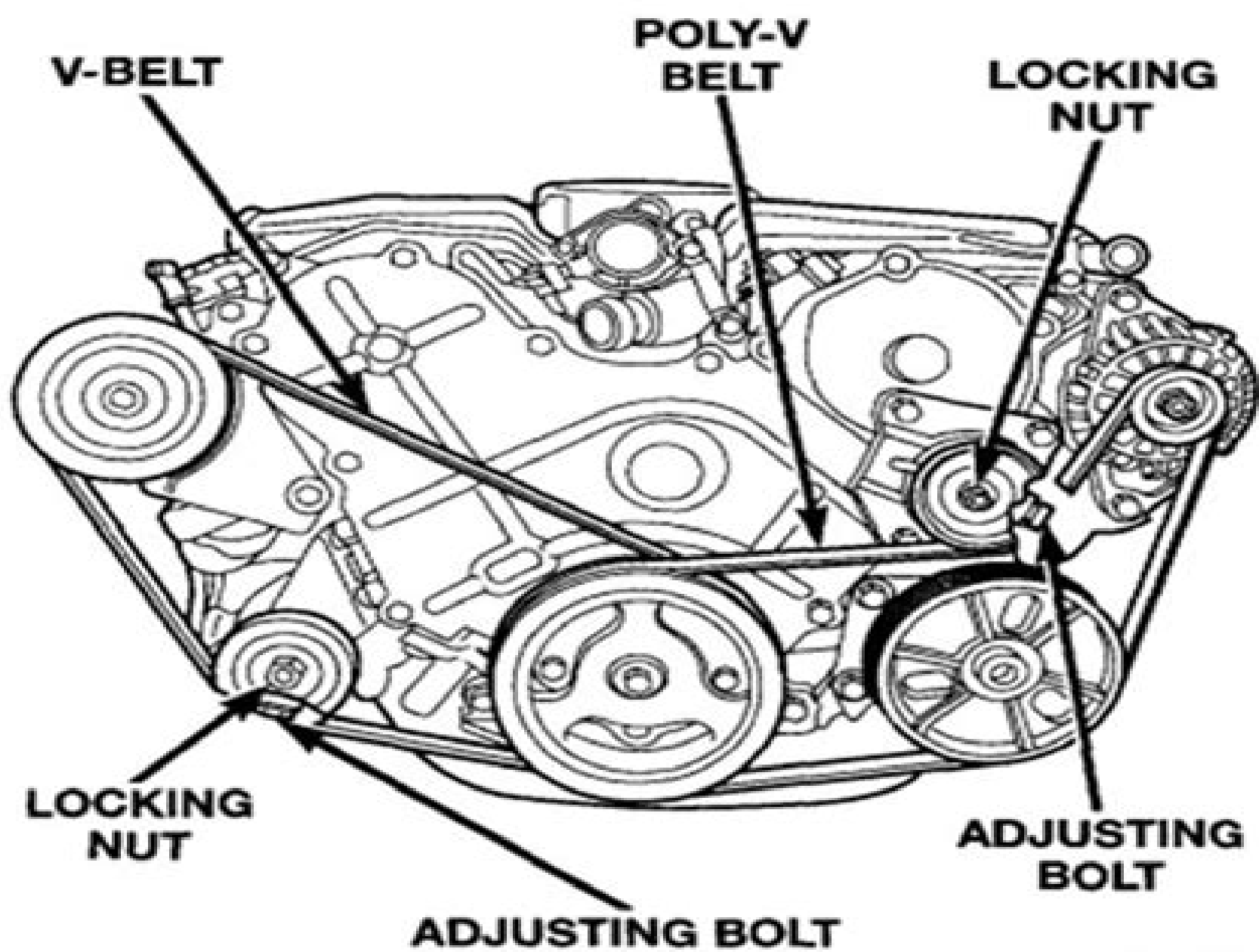
Fig. 36 Accessory Drive Belts
