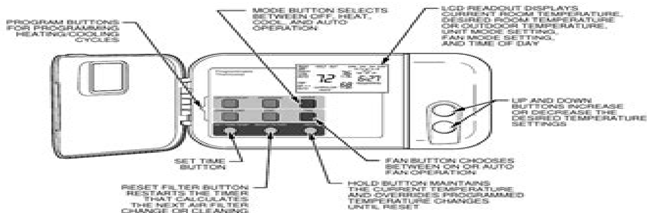
Fig. 3—Carrier Programmable Thermostat
