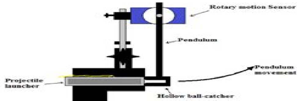
Figure 1. Ballistic pendulum setup.
