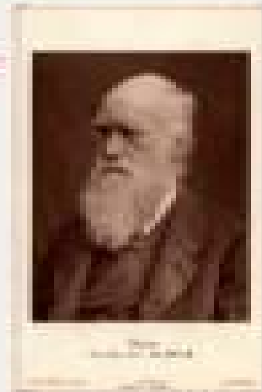
Figure 3.10 Darwin's portrait
