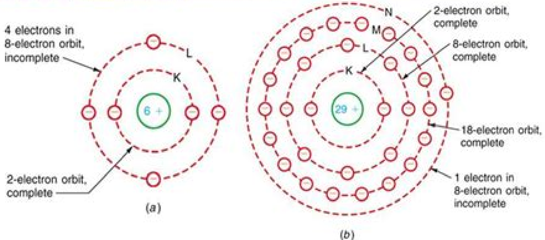
Fig. 1-3: Atomic structure showing the nucleus and its orbital rings of electrons. (a) Carbon (C) atom has 6 orbital electrons to balance 6 protons in the nucleus. (b) Copper (Cu) atom has 29 protons in the nucleus and 29 orbital electrons.
