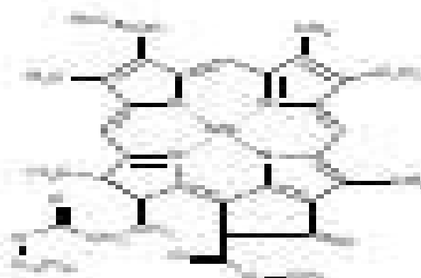
Chemical structure 1
