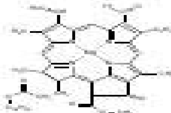
Chemical structure 2
