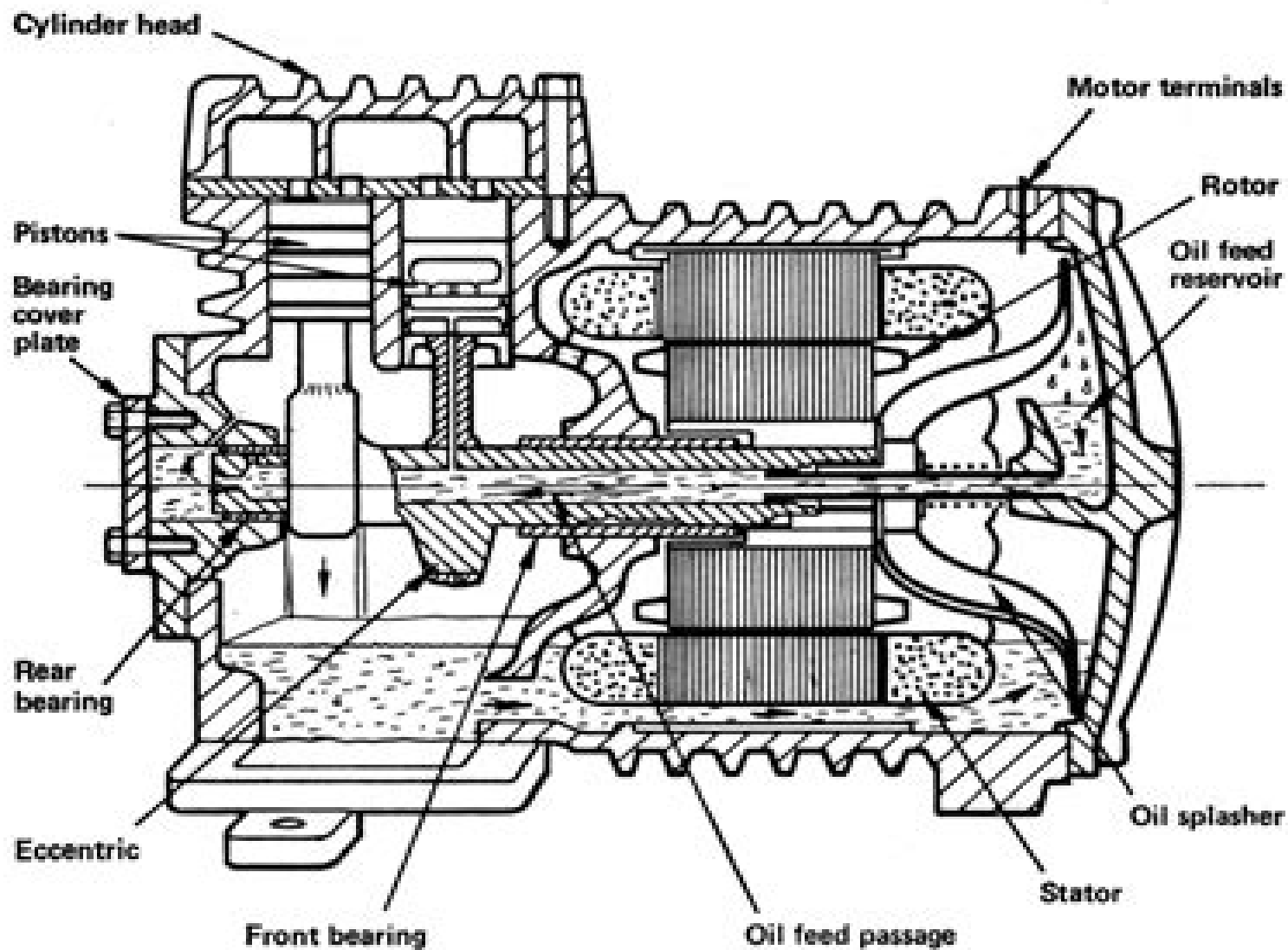
Fig. 2—Sectional view of a semi-hermetic compressor.
