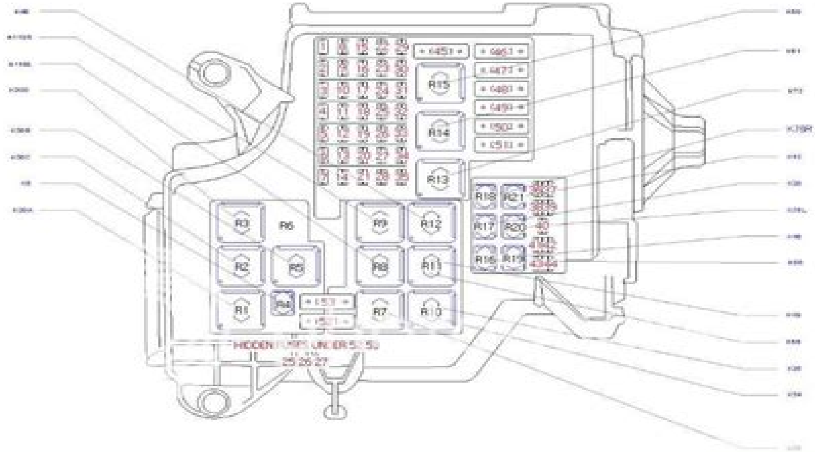
Relays and Fuses Corsa C, model year 2002
