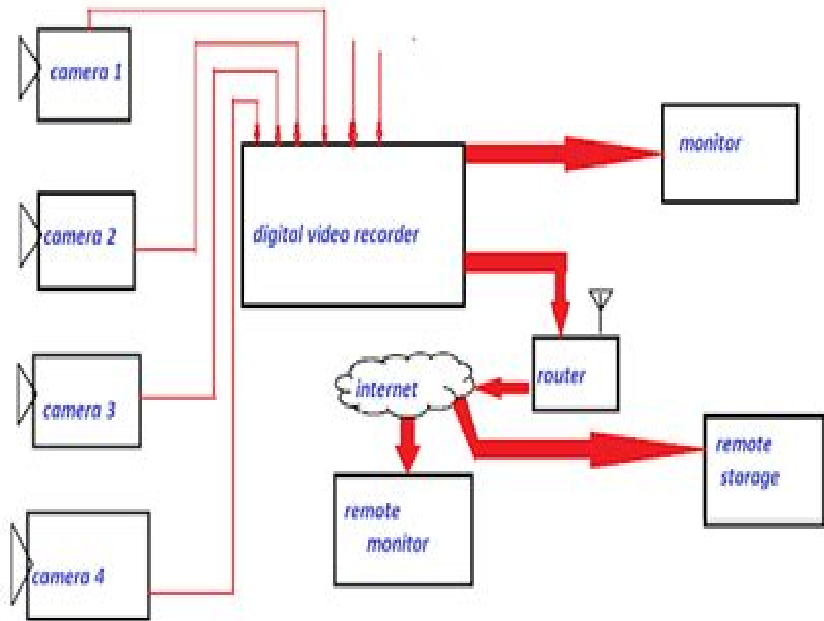
BLOCK DIAGRAM OF CCTV SYSTEM
