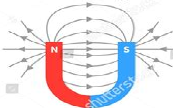
Horseshoe magnet
