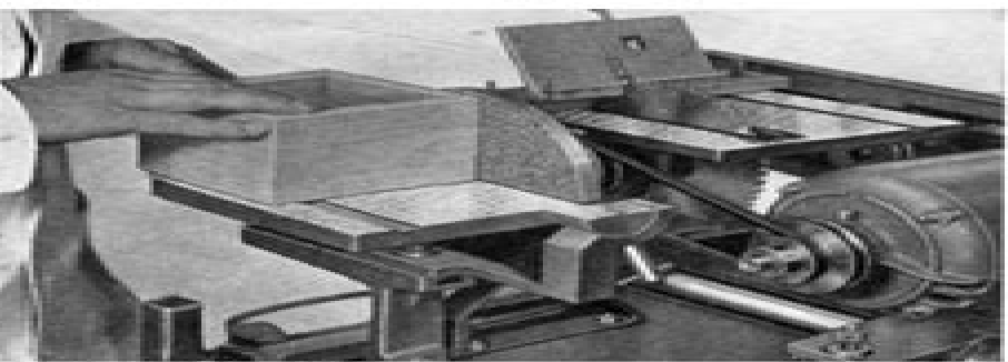
DISC-SANDING. This large size 8 in. sander is an improved type, incorporating tilting table with mitre fence, permitting the sanding of all compound angles. (Standard Unit plus M520, M10a).
