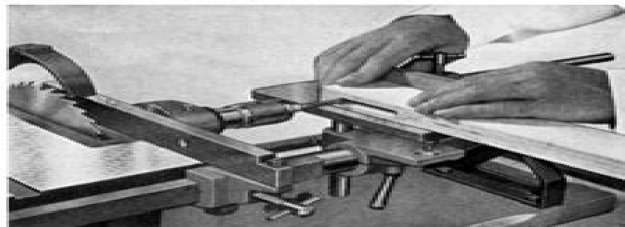
MORTISING. This operation speedily and accurately carried out using variable height combination table, slot miller chuck and bit. (Standard Unit).
