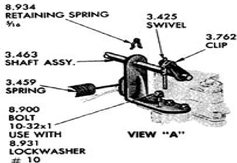
1960-62 CORVAIR—F.C. CARBURETOR LINKAGE (TYPICAL)
