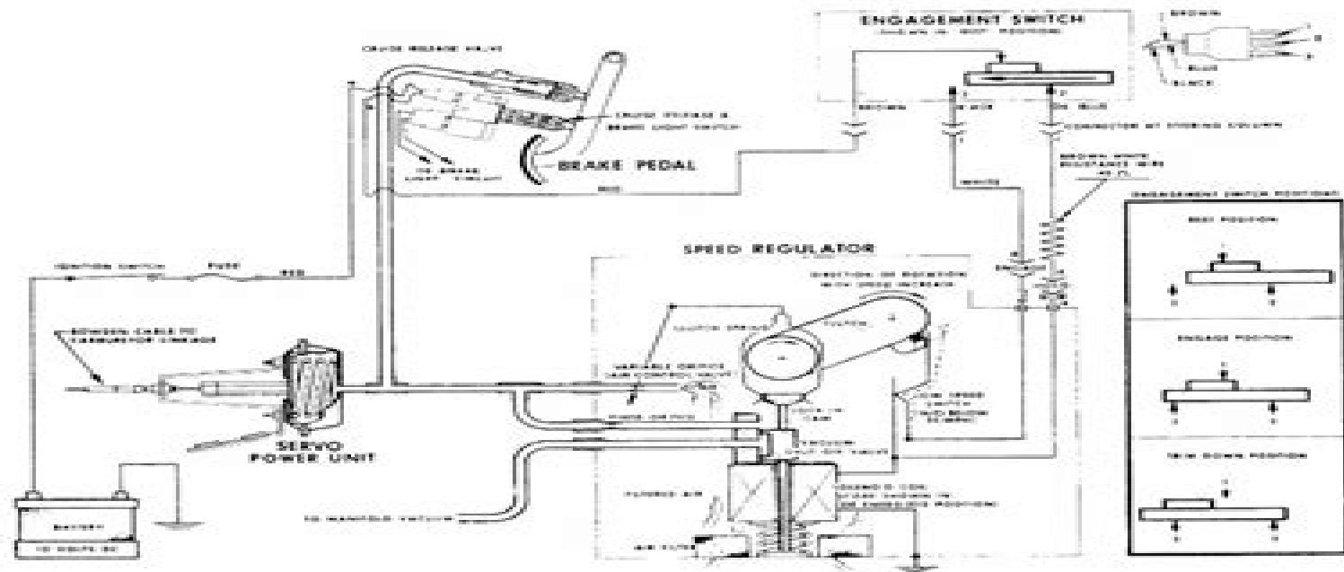
General Motors Cruise Master Automatic Speed Control System Wiring Diagram
