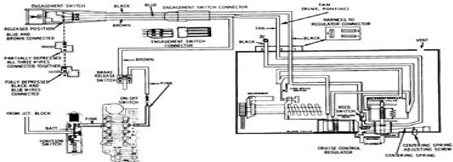
General Motors Cruise Control Automatic Speed Control System Wiring Diagram
