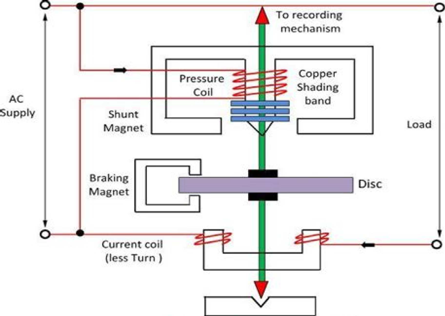
Induction Type Energy Meter
