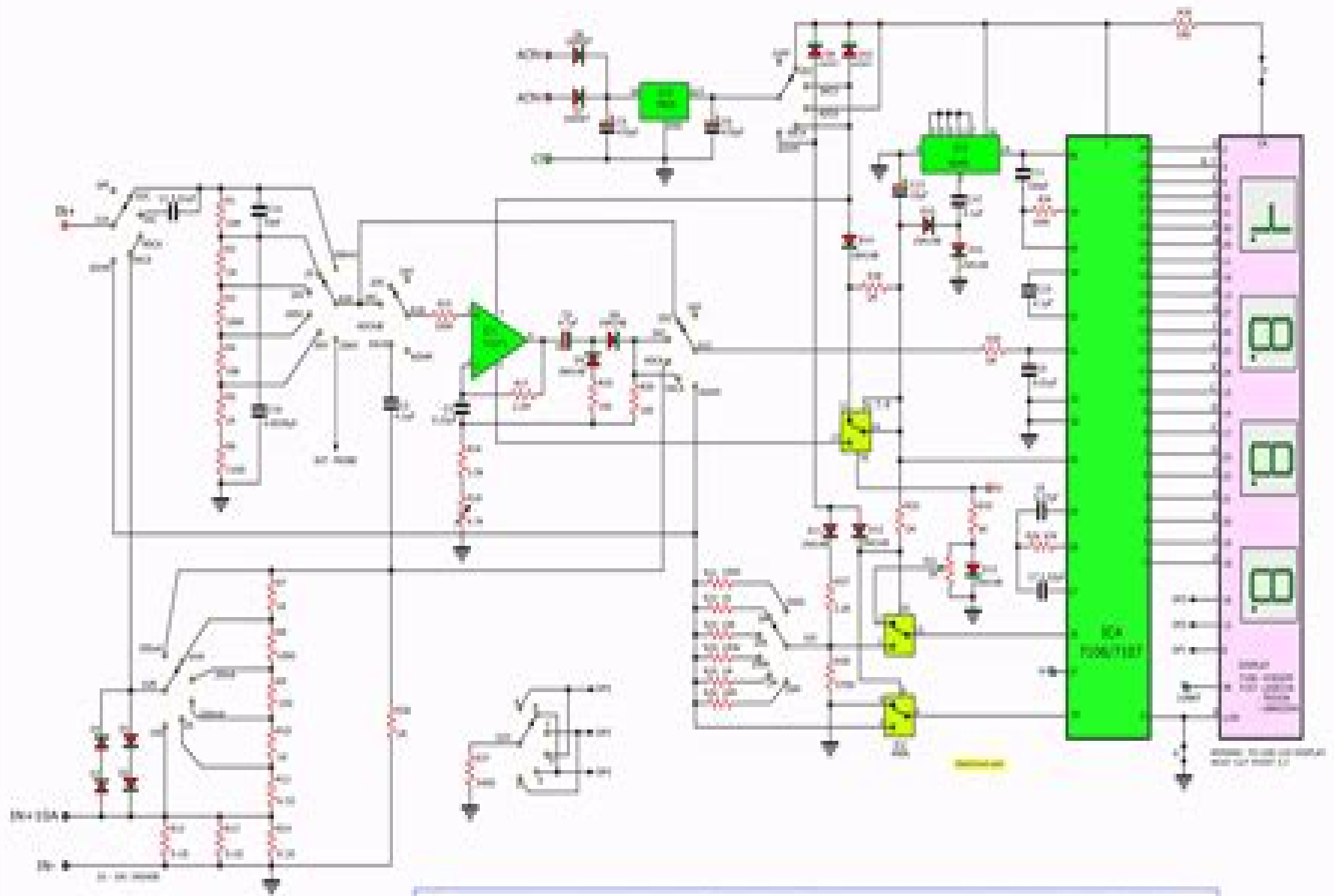
Digital Multimeter Circuit Diagram using 7107 / 7106
