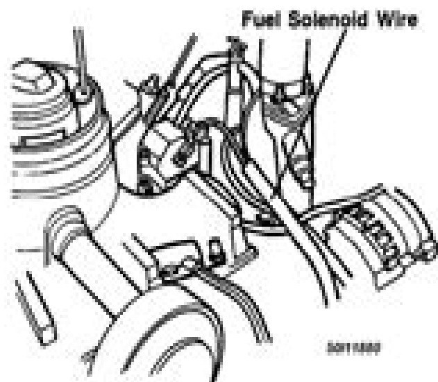
Fig. 8: Fuel Injection Pump Solenoid (Diesel) Courtesy of GENERAL MOTORS CORP.
