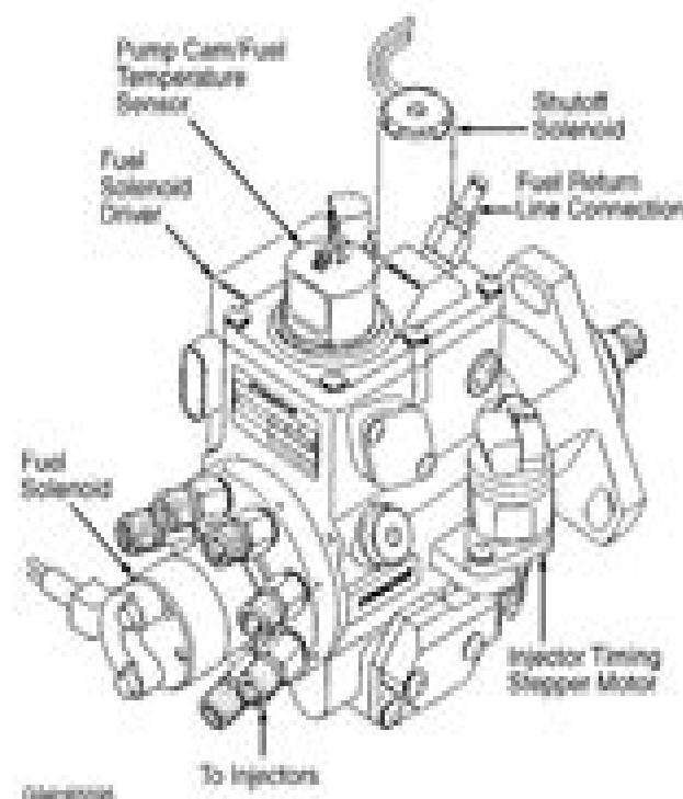
Fig. 9: Identifying Diesel Injection Pump Components Courtesy of GENERAL MOTORS CORP.
