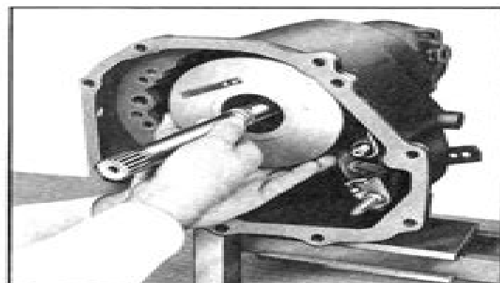
Fig. 117—Installing Unit Assembly into Case
