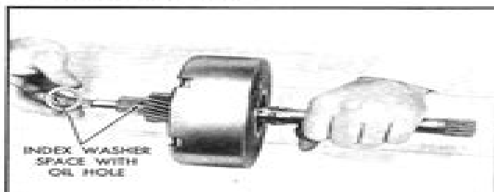
Fig. 114—Alignment of Thrust Washer Oil Slot with Shaft Oil Hole
