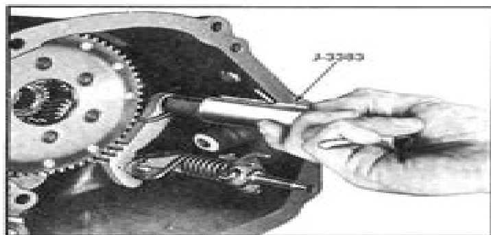
Fig. 115—Installing Parking Pawl Spring
