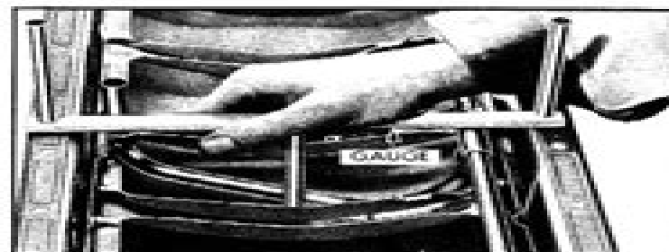
Fig. 24—Checking Oil Trough Depth
