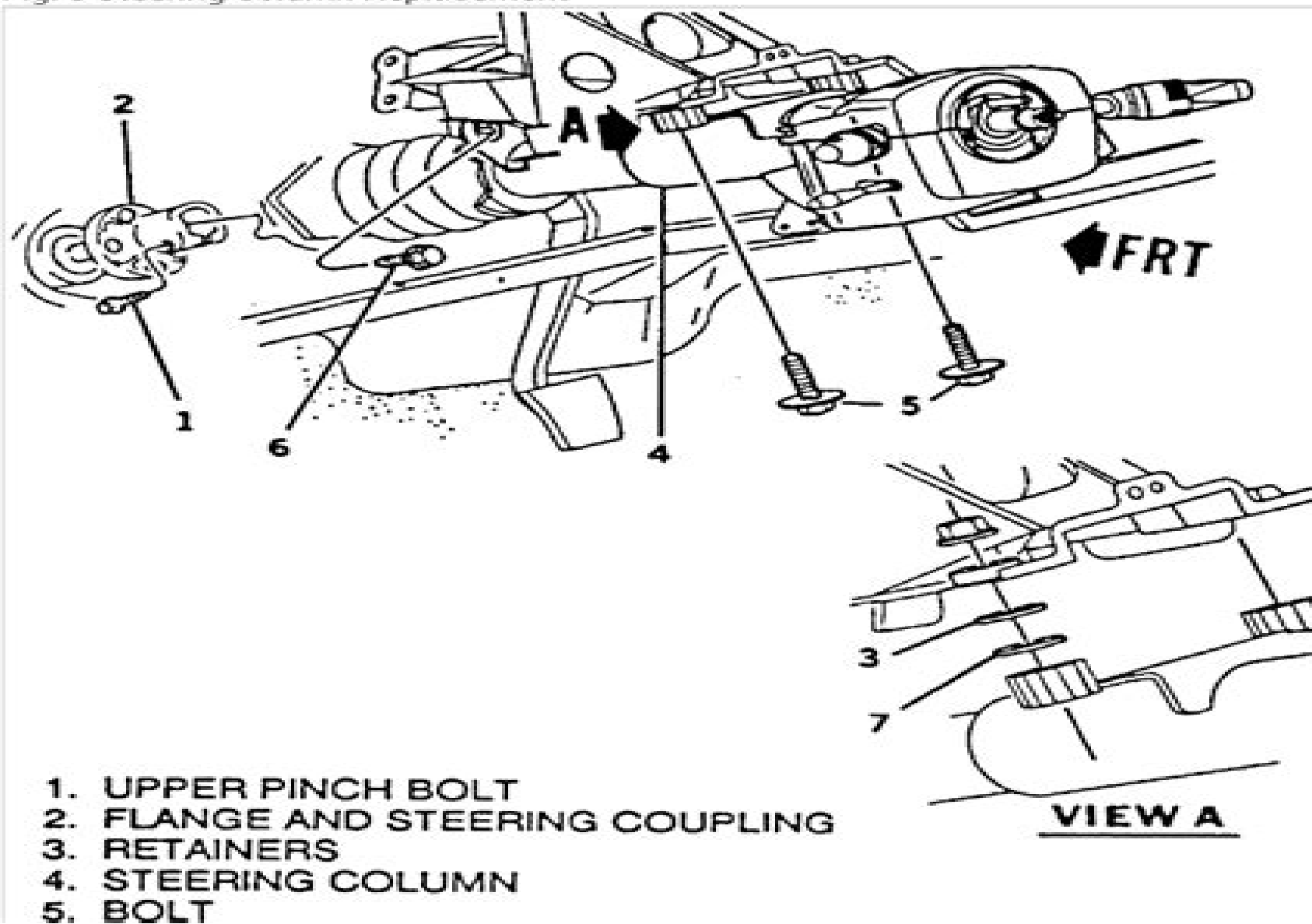
Fig. 3 Steering Column Replacement
