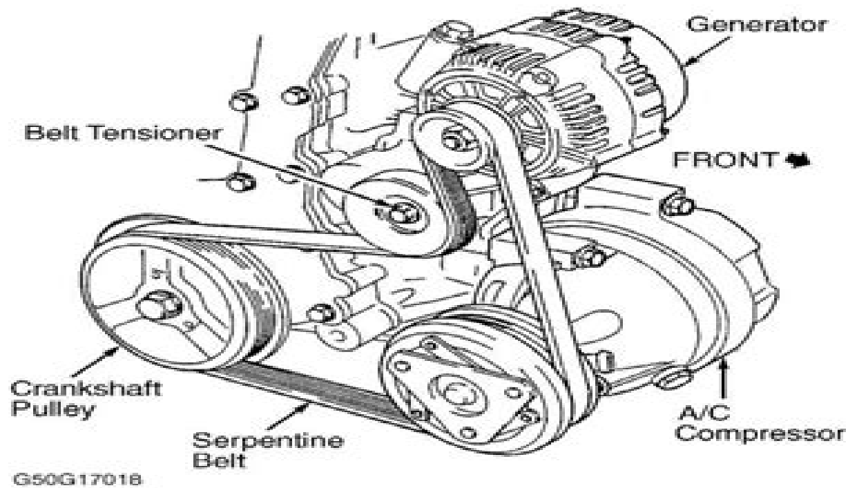
Fig. 11: Serpentine Belt Routing (2.4L Cavalier & Sunfire) Courtesy of GENERAL MOTORS CORP.
