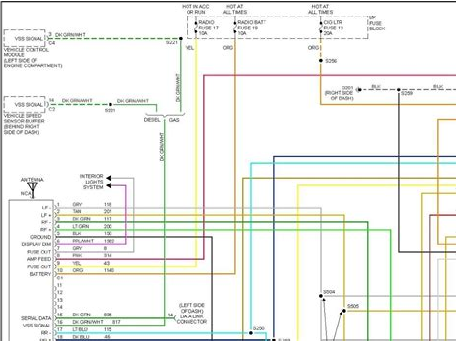
1995 GMC Truck Fig. 33: Radio Controls, UHF Amplifier
