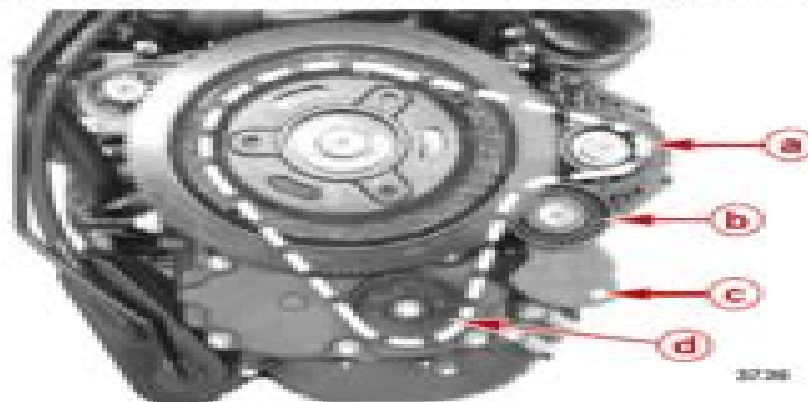
a - Alternator b - Tensioner pulley c - Tensioner release slot d - Supercharger
