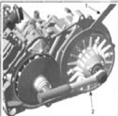
1 Clutch holding tool 2 Driven pulley
