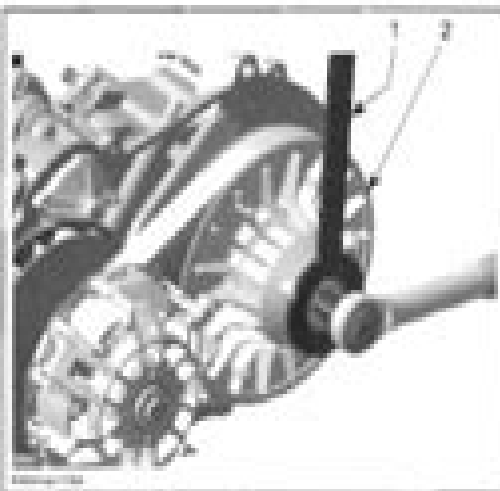
1 Clutch holding tool 2 Driven pulley (fixed half)
