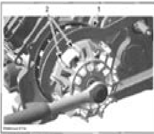
1 Clutch holding tool 2 Driven pulley (transmission side) view
