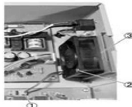
1 Connector 2 Screw 3 Cooling fan
