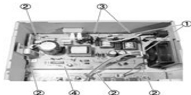
1 Connector 2 Screw 3 Fitting part 4 Power supply PCB
