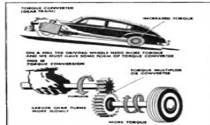
Fig. 44—Torque Requirement (Hill)
