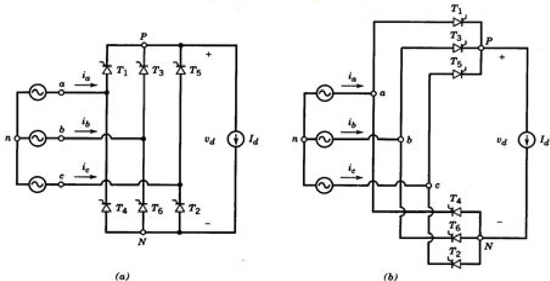
Figure 6-19 Three-phase thyristor converter with L_a = 0 and a constant dc current.
