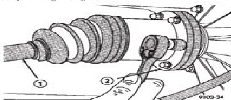
Fig. 2 Half Shaft Mounting Bolts
