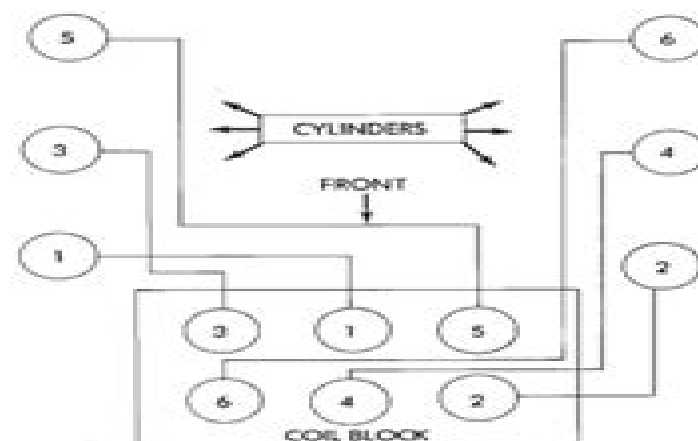
Fig. 1 Spark Plug Wire Routing—3.3L and 3.5L Engine
