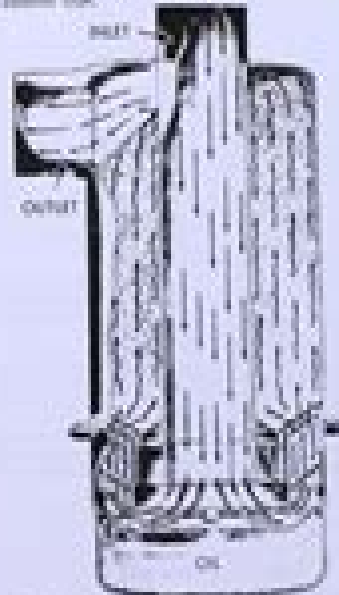
Figure 20 — Sectional View of Oil Bath Air Cleaner
