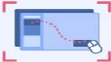
Software Simulation
